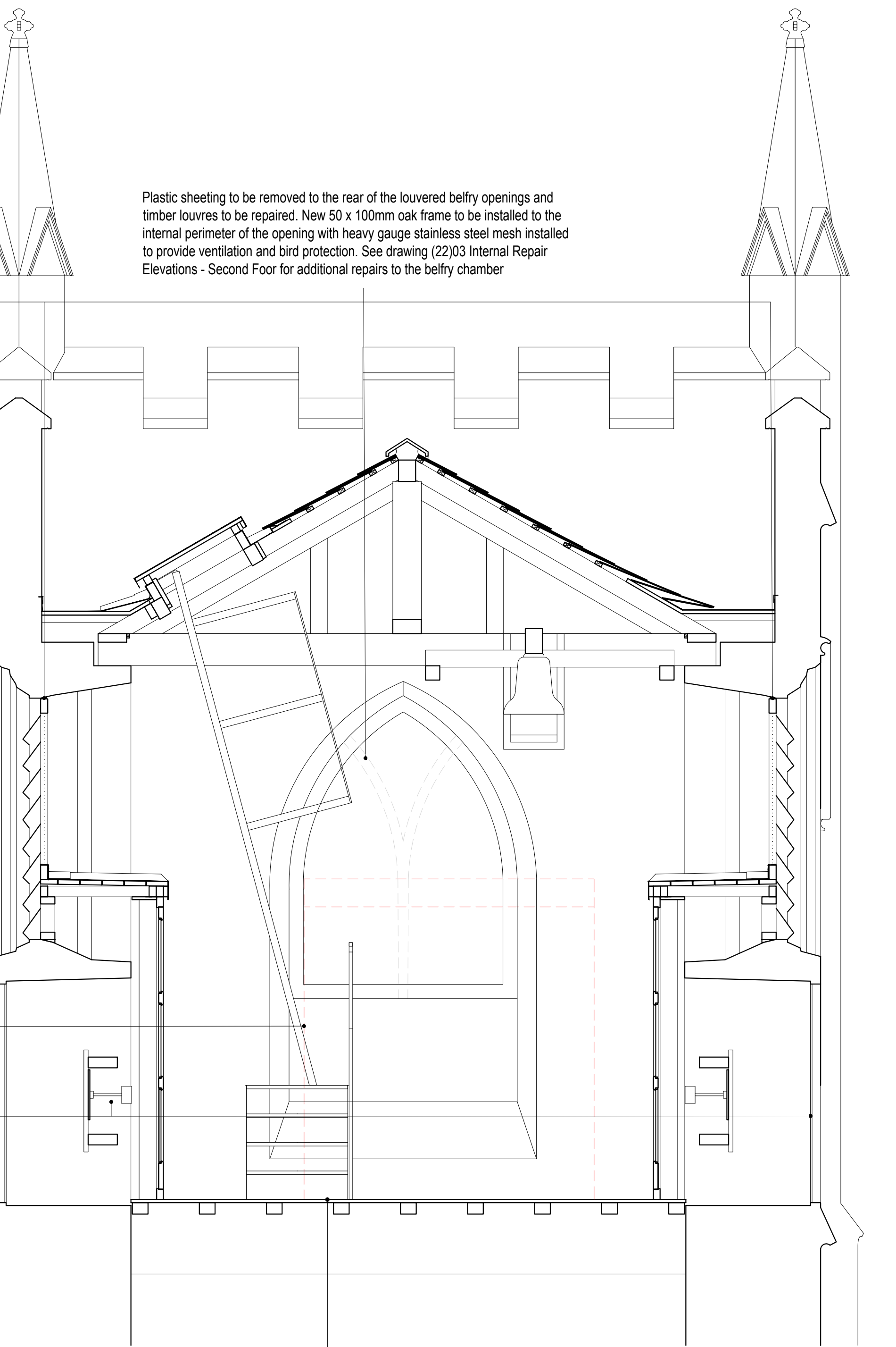
2 SECTION BB AS PROPOSED (30)02 1:25
