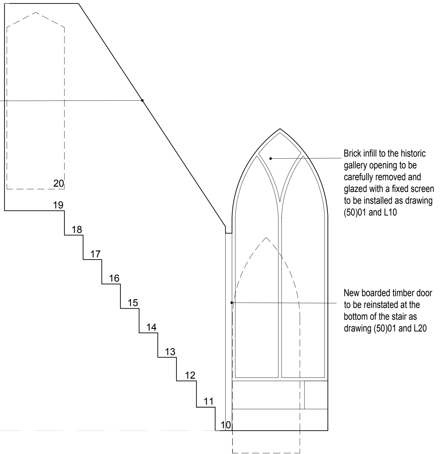
3 SECTION CC AS PROPOSED (30)02 1:25
