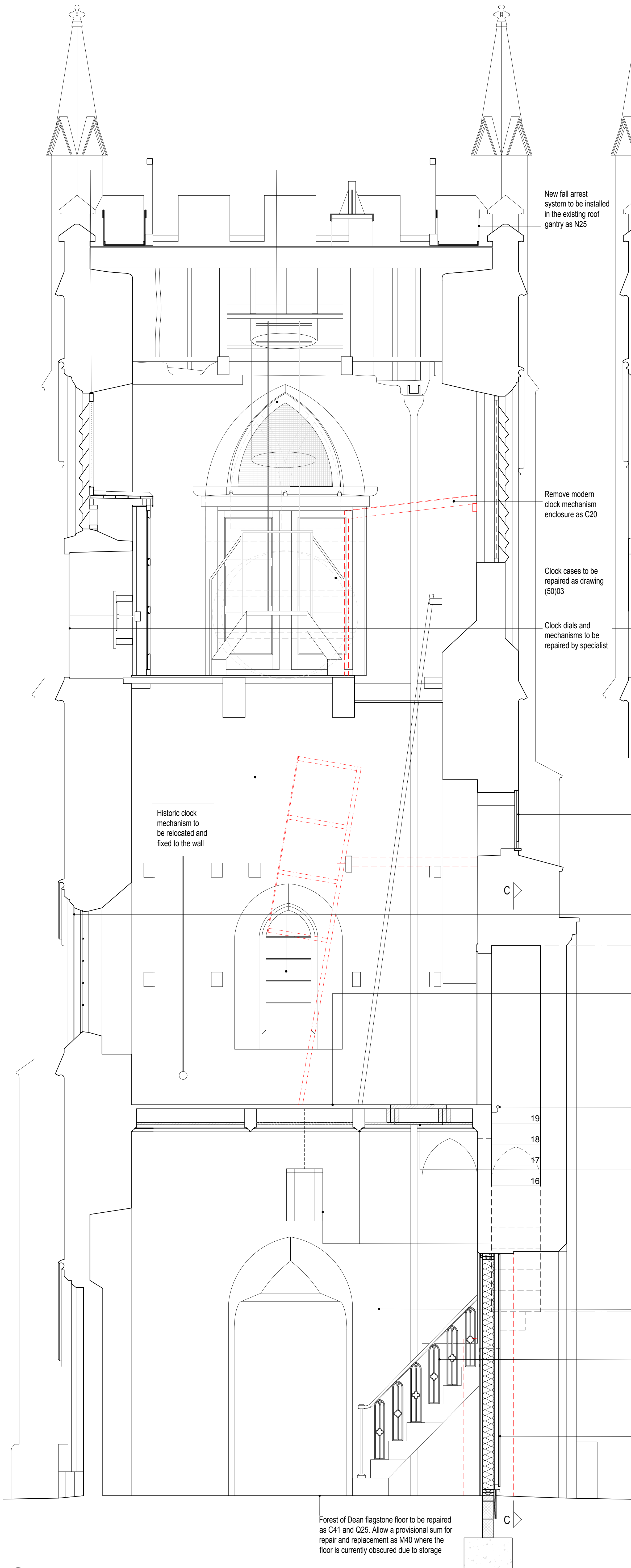
1 SECTION AA AS PROPOSED (30)02 1:25
